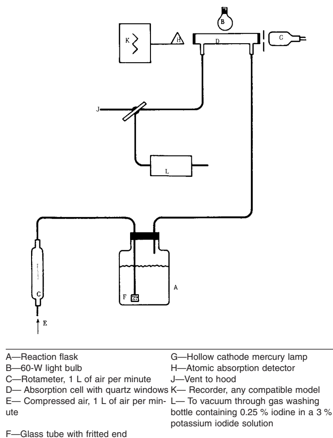
FIG. 2 Schematic Arrangement of Equipment for Mercury Measurement by Cold Vapor Atomic Absorption Technique Open One-Pass System
