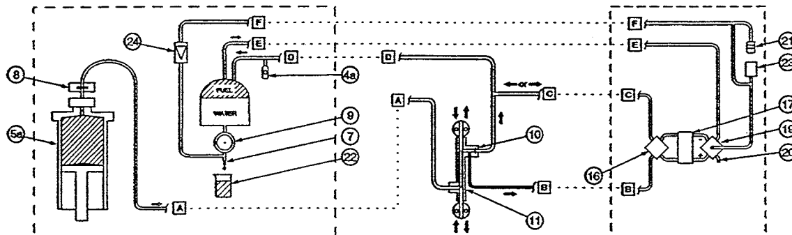
230 Type—hydraulically pressurized / syringe pump / differential transducer / standard test section
