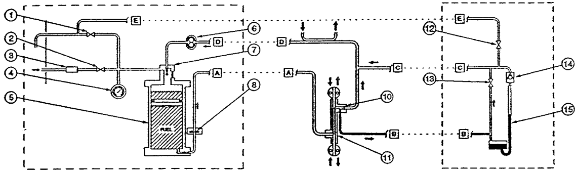
203 Type—pneumatically pressurized / gear pump / mercury manometer / standard test section
