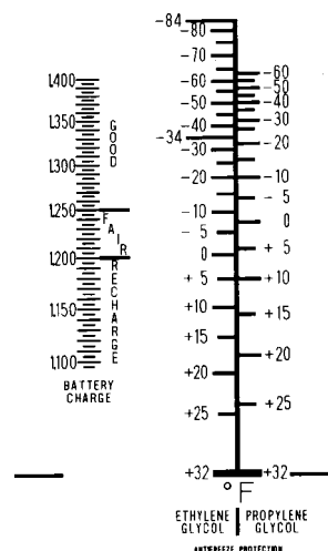
FIG. 5 Tester Temperature Scale
