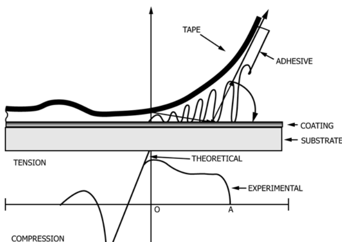
FIG. X1.1 Peel Profile (6)
