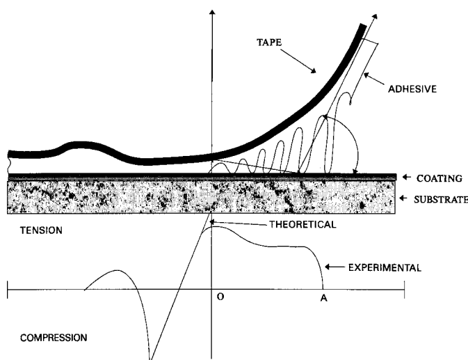
FIG. X1.1 Peel Profile (6)
