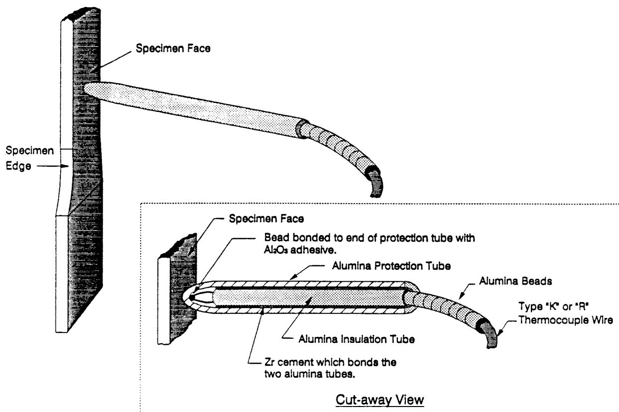
FIG. 7 Sheathed Thermocouple
