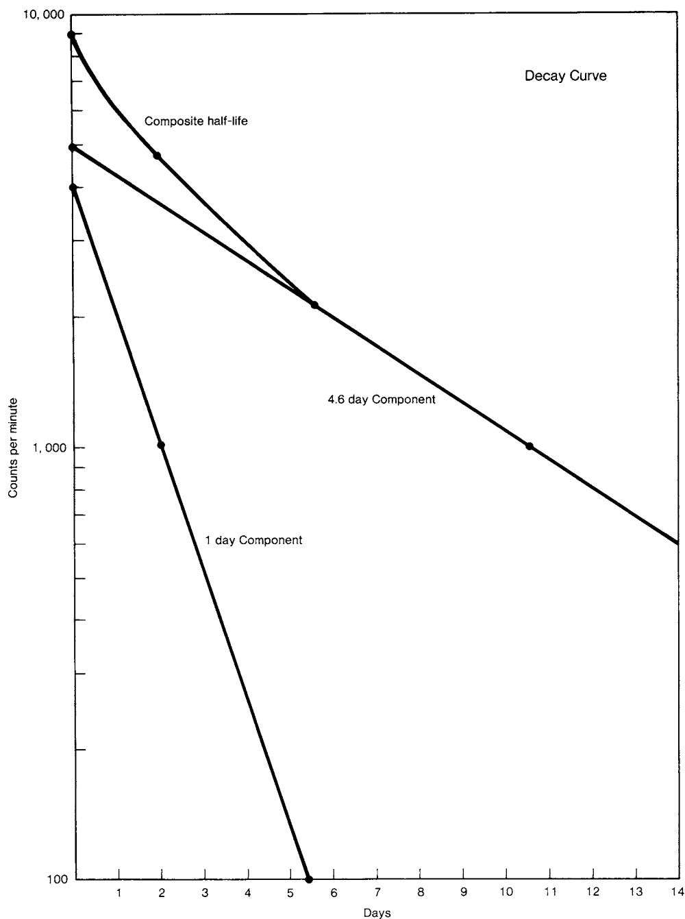
FIG. 8 Decay Curve
