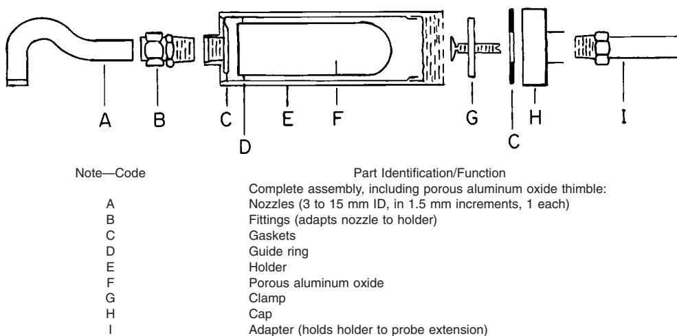
FIG. 4 Thimble Holder
