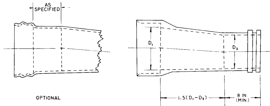
FIG. 2 Eccentric Reducer
