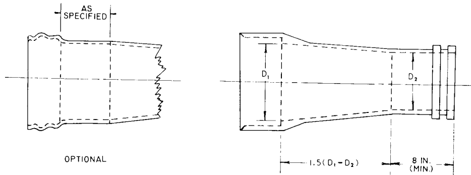
FIG. 1 Concentric Reducer
