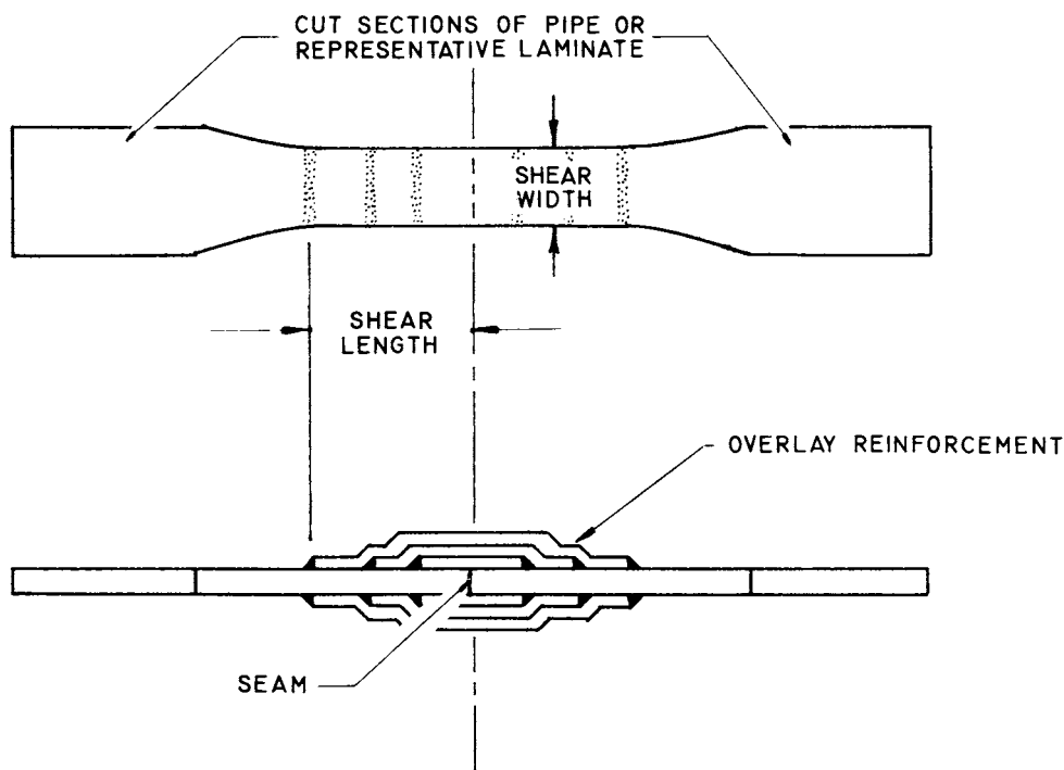
FIG. 3 Shear Test Specimen
