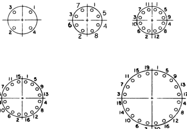
FIG. 2 Bolt Torquing Sequence
