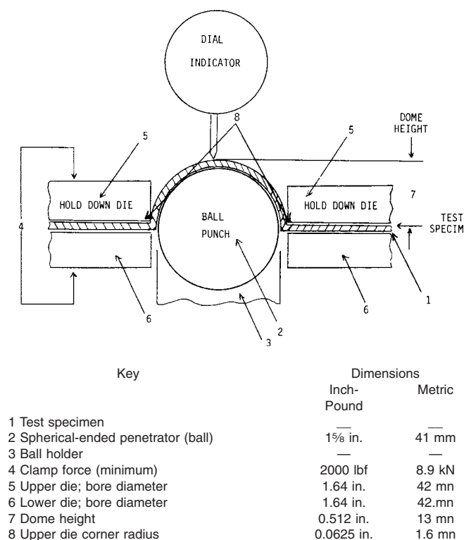
FIG. 2 Tooling for Forming Test
