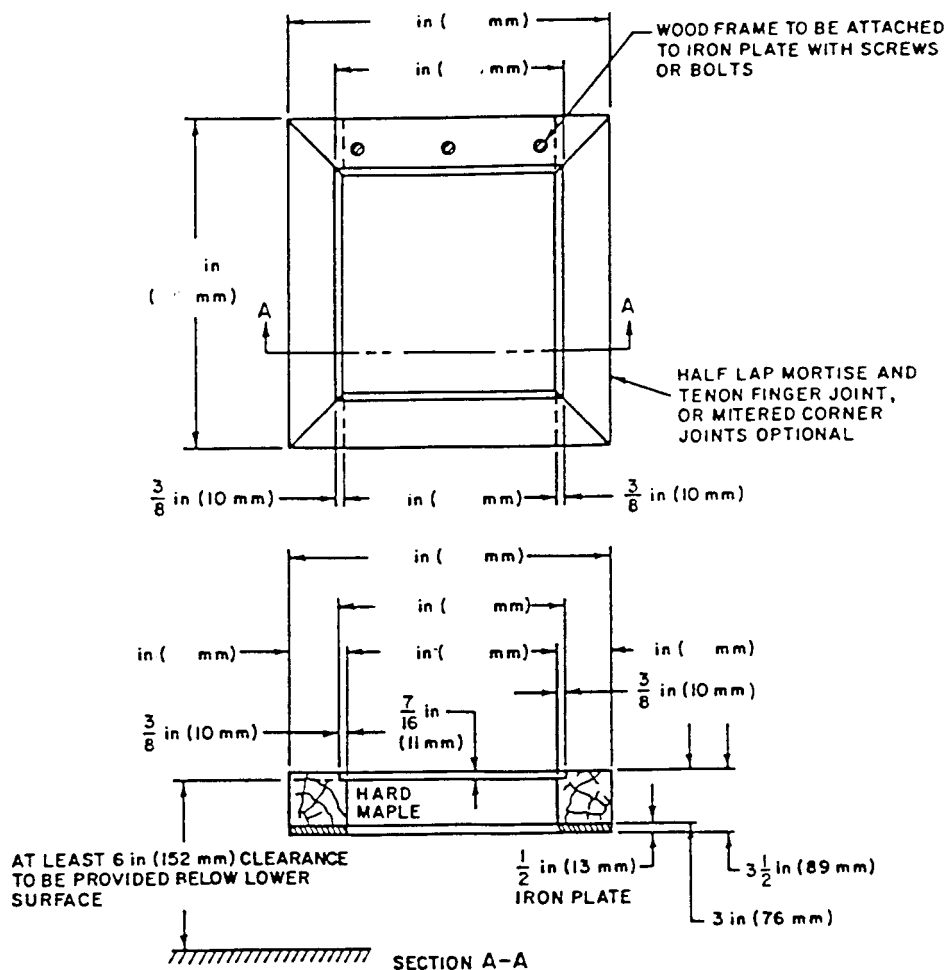
FIG. A2.1 Wood Holding Fixture for Drop Test
