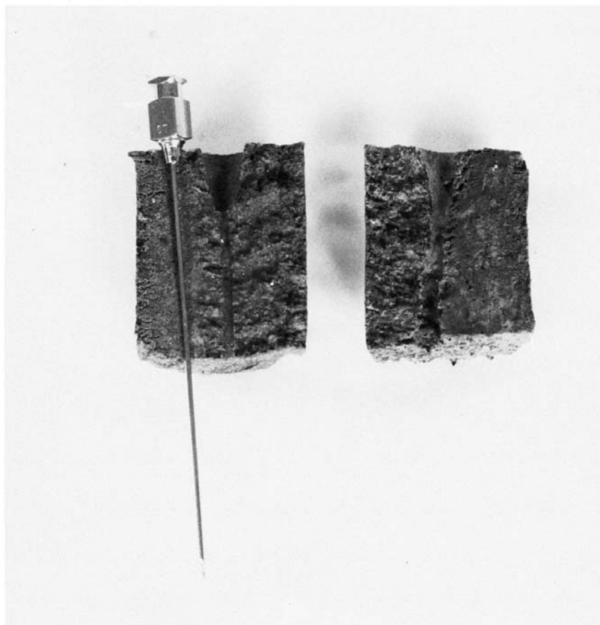
FIG. 5 Appearance of Typical Clay Pinhole Specimens After Completion of Test
