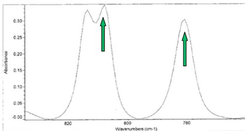
FIG. 1 IR Scan of TDI Showing 2,4-TDI Isomer Doublet at 810 \text{cm}^{-1} and 2,6 TDI Isomer at 782 \text{cm}^{-1}
