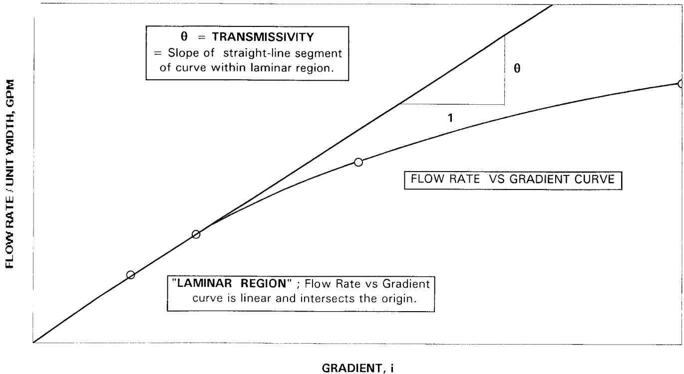
FIG. X1.1 Hydraulic Transmissivity
