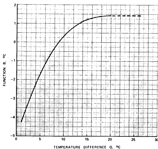
FIG. X2.2 Function B versus Distillation Temperature Difference Q
