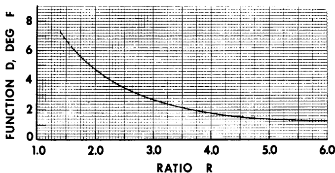
FIG. X2.8 Function D versus Ratio R
