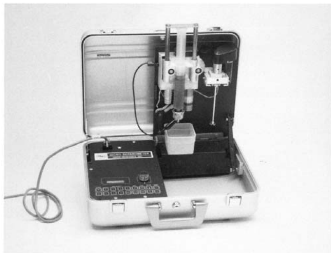
FIG. 4 Syringe Assembly in Syringe Drive
