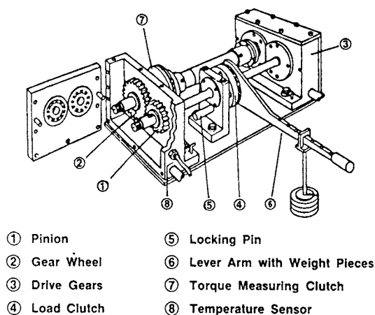
FIG. A2.1 FZG Gear Oil Test Machine
