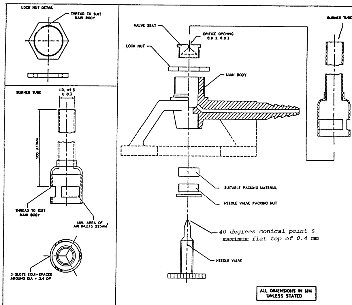
FIG. 1 Burner Design
