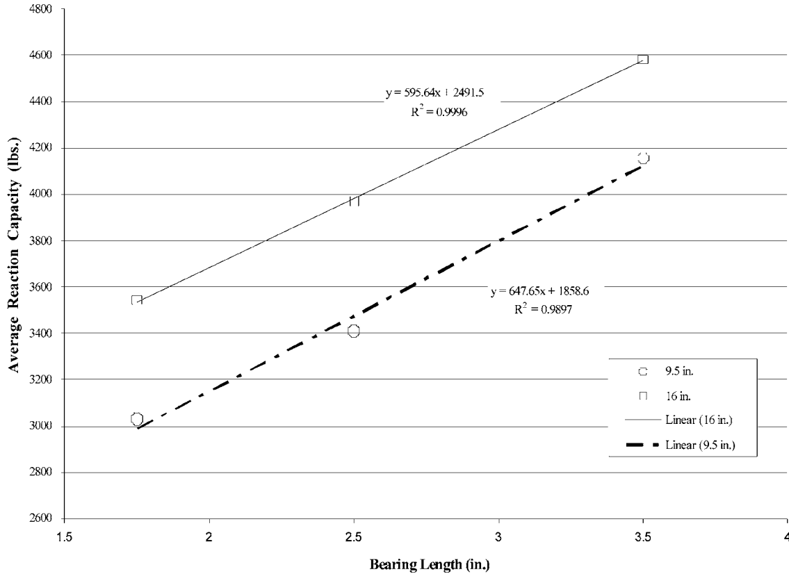
FIG. X8.1 Mean Reaction Capacities
