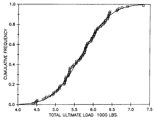
FIG. X4.1 11.875 Data and Normal Distribution
