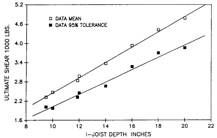
FIG. X4.2 Correlation of Shear Strength and Depth
