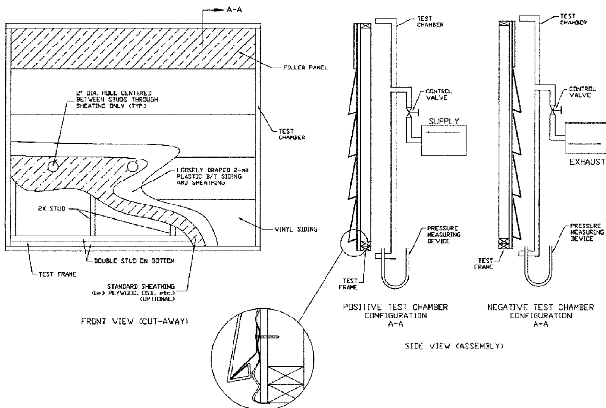
FIG. 1 Test Chamber
