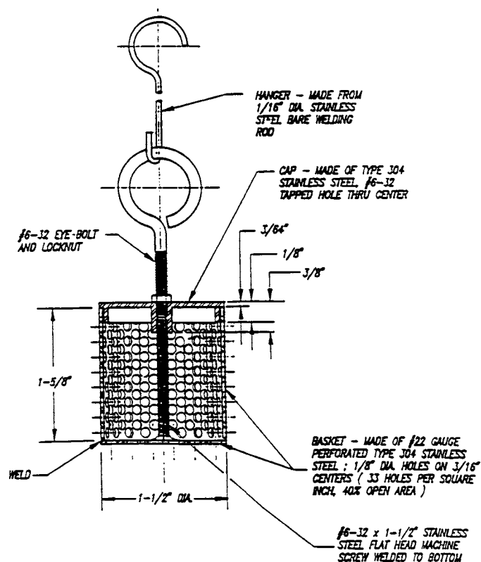
FIG. X1.1 Basket for n -Hexane Extractables 1
