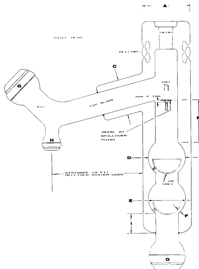
STILL HEAD DIMENSION CHART
