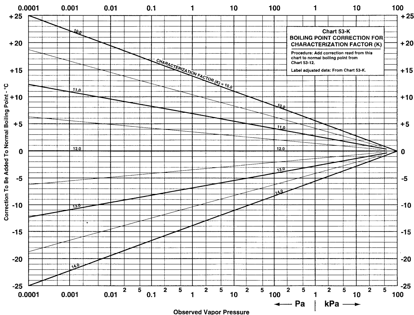
FIG. A4.2 Boiling Point Corrections for K -Factor
