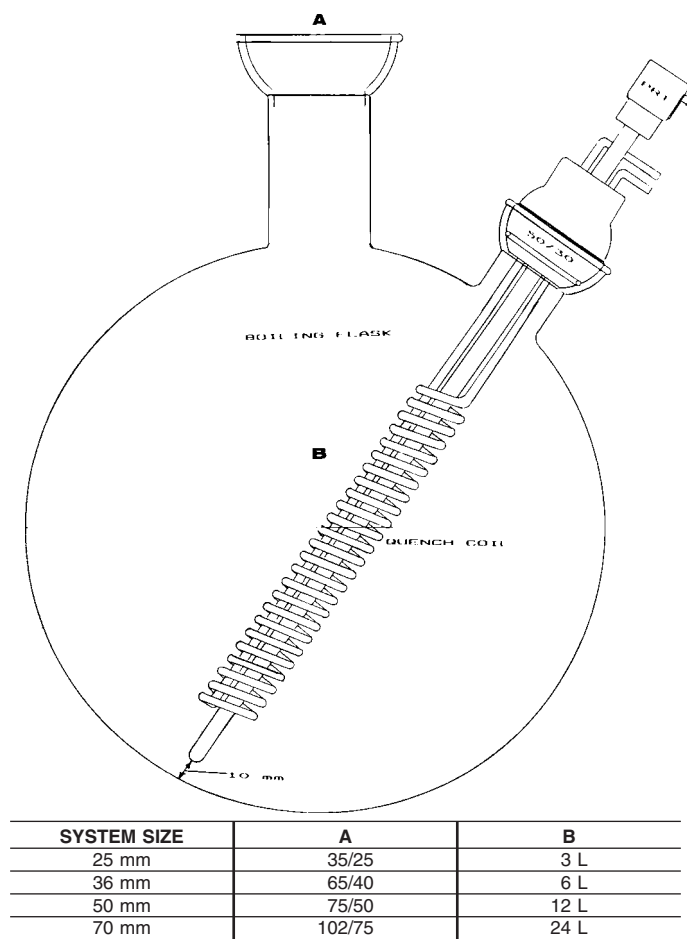
FIG. 3 Distillation Flask
