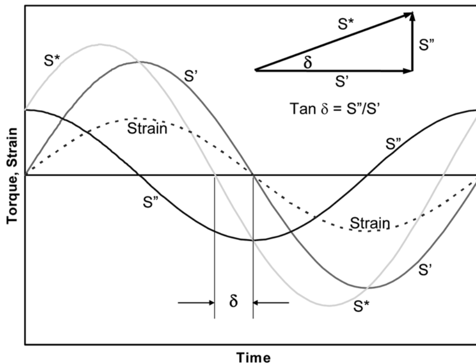
FIG. 2 Example of Torque Responses for an Oscillation Cycle
