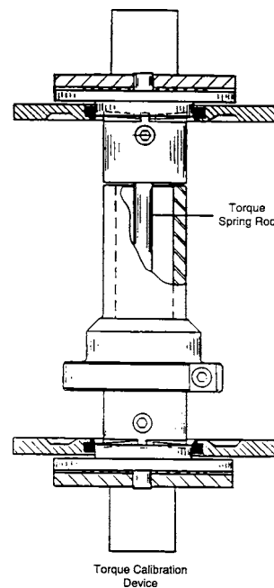
FIG. 6 Typical Torque Standard Calibration Device for Torsion Shear Curemeters
