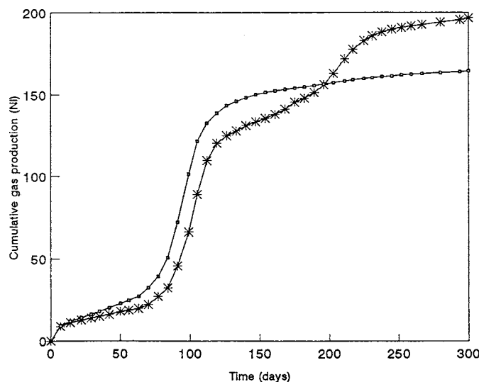
FIG. 2 Cumulative Biogas Production Over a Period of 300 Days for 1 kg of Pretreated Household Waste Plus 100 g of Mesophilic Anaerobic Inoculum Without Sample (Blank) and With 60 g of Cellulose (Plus Positive Control)
