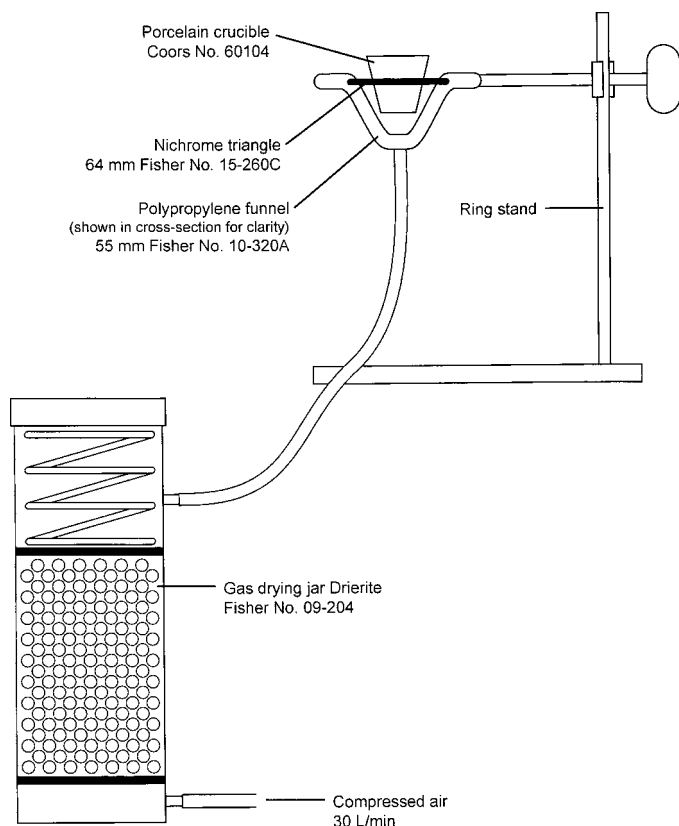
FIG. 1 Cooling Assembly
