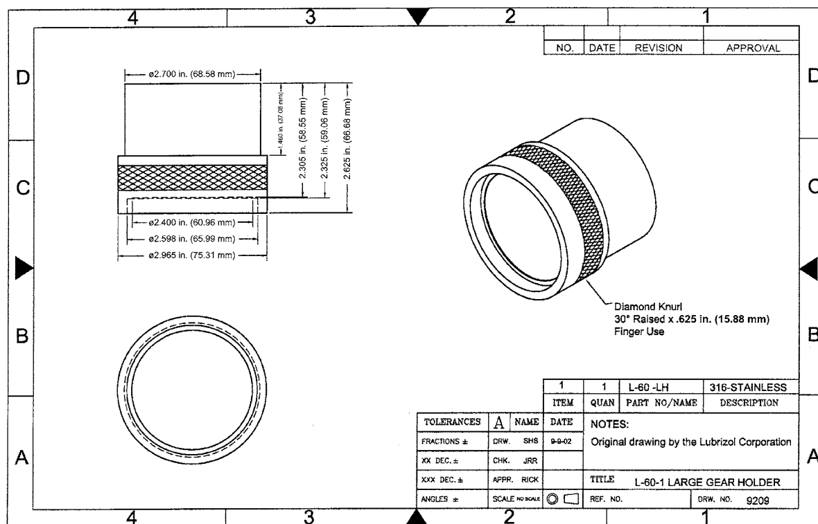
FIG. A9.2 Large Gear Holder
