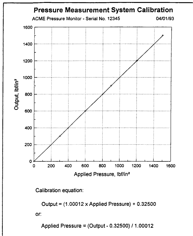
FIG. X1.1 Example Least-Squares Line Plot
