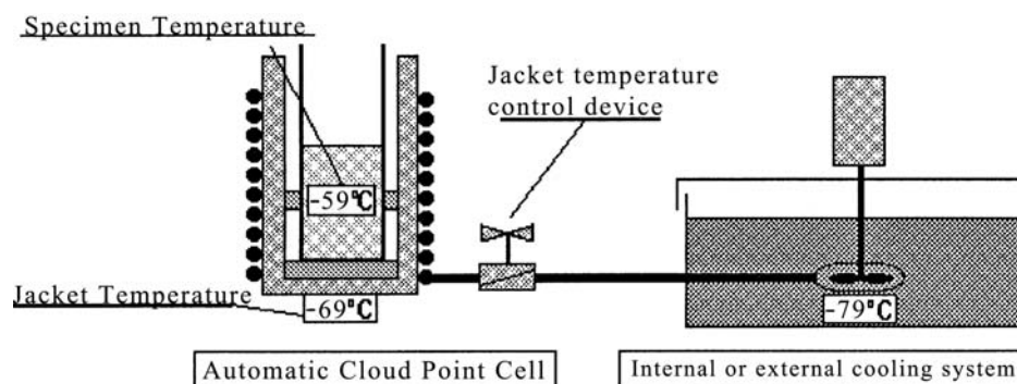
FIG. 3 Test Jar Cooling Chamber and Cooling System
