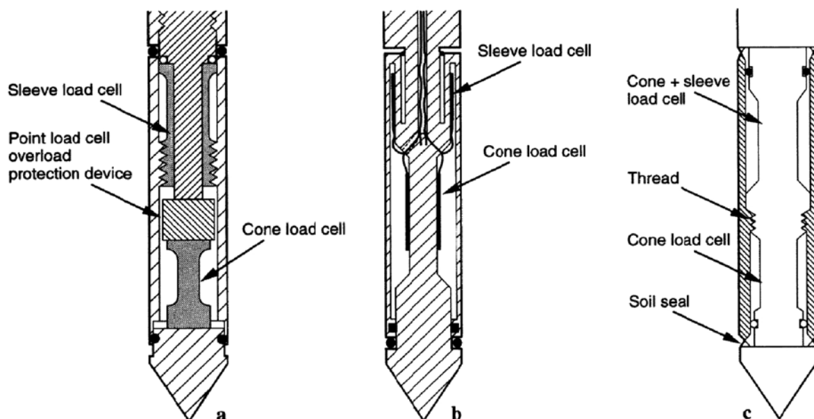
FIG. 1 Common Configurations for Electric Friction-Cone Penetrometers (4) Showing: (a) Compression-type Tip and Sleeve Load Cells, (b) Tension-type Sleeve Design, and (c) Subtraction-type Penetrometer
