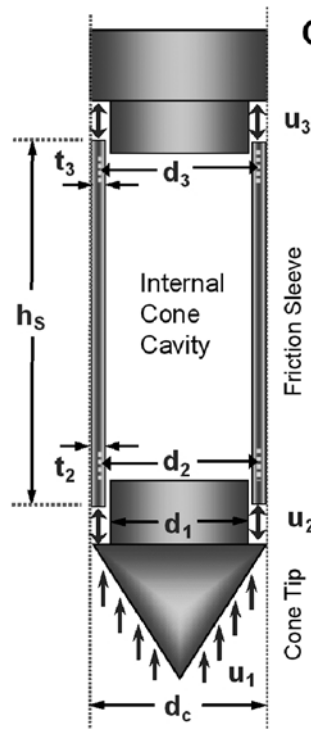
FIG. A1.2 Schematic of Net Area Ratio ( a_n ) for Corrections of Cone Tip Resistances (6)
