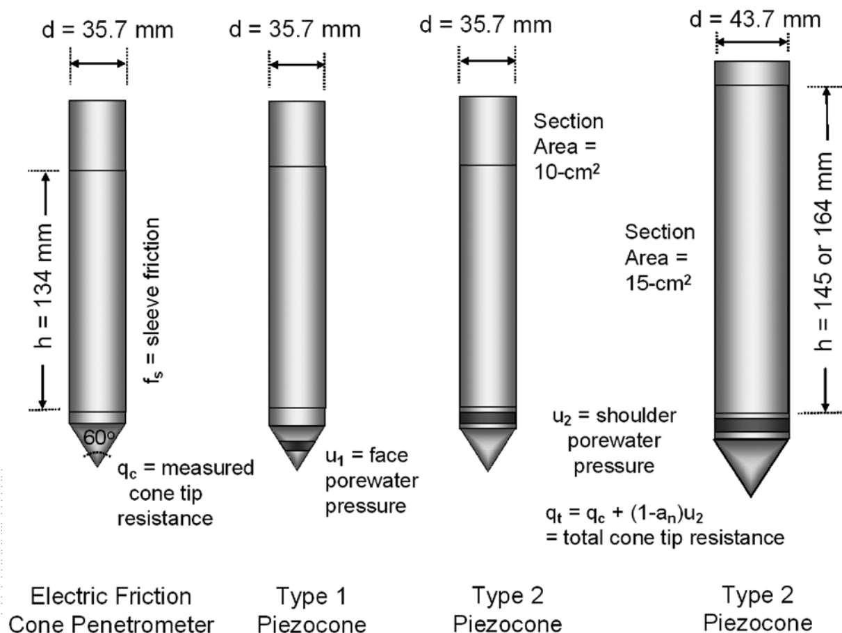
FIG. 3 Penetrometer Design Configurations: (a) Electronic Friction-type, (b) Type 1 Piezocone, (c) Standard 10-cm 2 Type 2 Piezocone, and (d) 15-cm 2 Type 2 Version (7)
