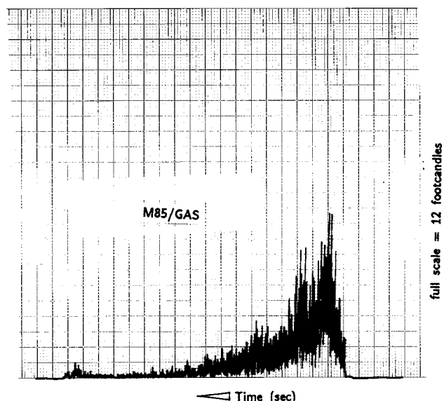
FIG. X2.3 Luminosity Trace of M85, 30 % Aromatic Gasoline
