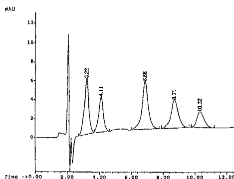
FIG. X1.1 Chromatogram 1
