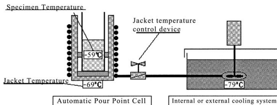
FIG. 2 Test Jar Cooling Chamber and Cooling System
