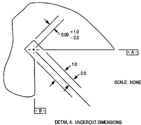
FIG. 21 Support Fixture-Short Grip Details (Inch-Pound)
