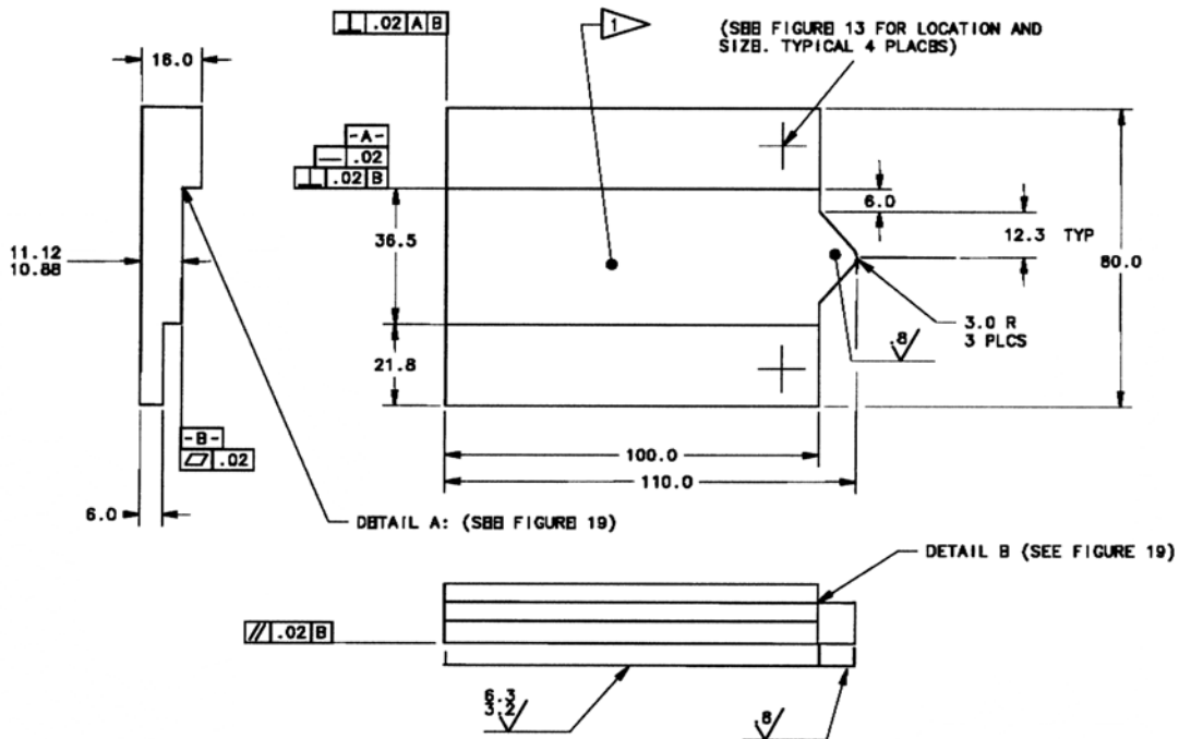
FIG. 19 Support Fixture-Long Grip Details (Inch-Pound)
