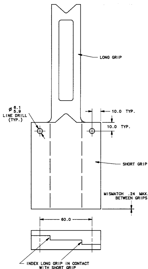
FIG. 16 Support Fixture-Line Drilling Details (SI)
