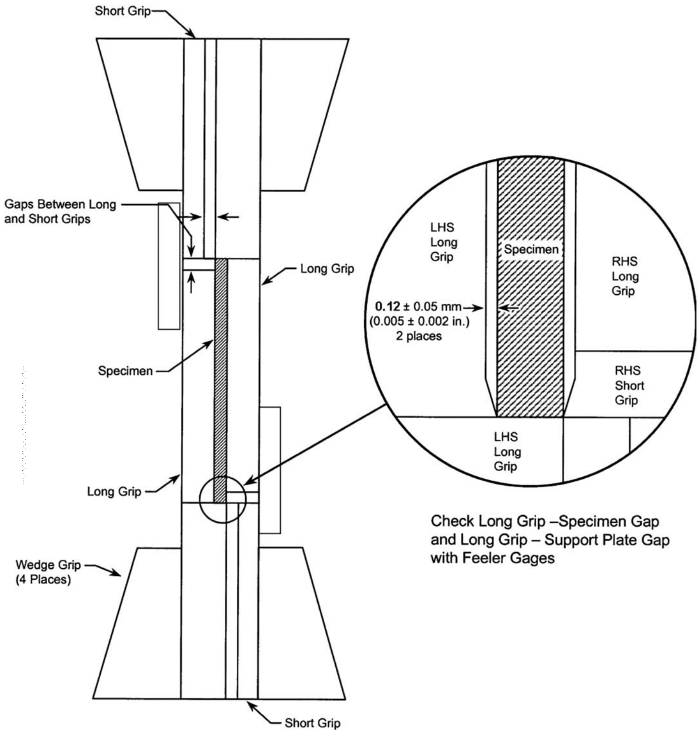
FIG. 28 Specimen/Support Fixture/Grip Assembly for Procedure B
