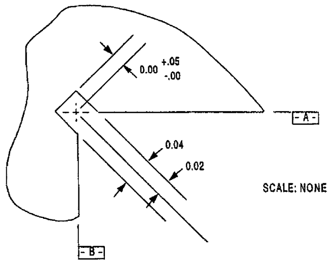
DETAIL A: UNDERCUT DIMENSIONS
