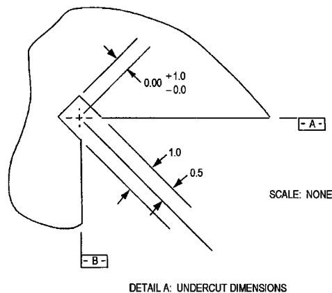
DETAIL A: UNDERCUT DIMENSIONS
