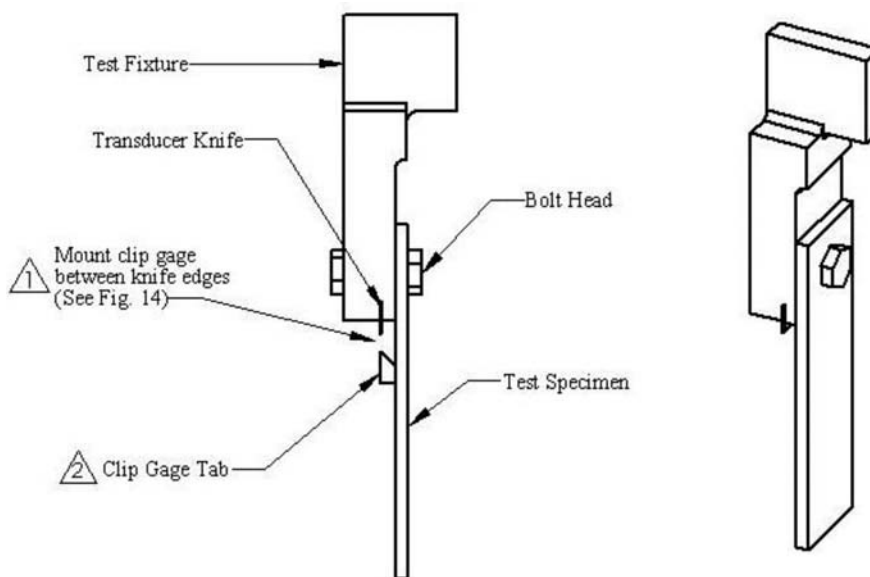
FIG. 10 One-Piece Single-Shear Test Fixture for Procedure C
