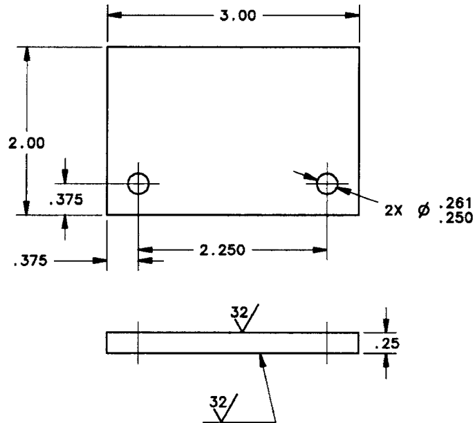
FIG. 25 Support Fixture-Support Plate Details (Inch-Pound)
