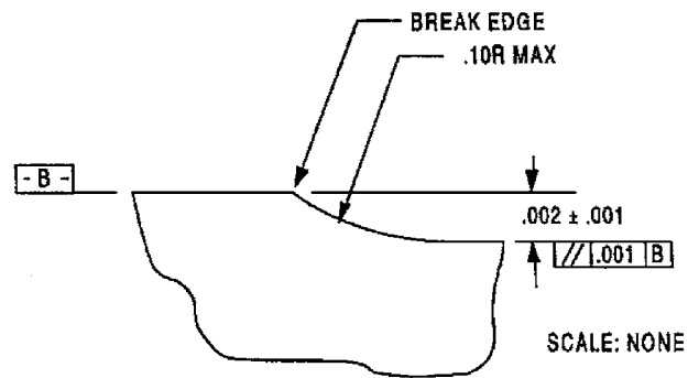
DETAIL B: RADIUS DETAIL
