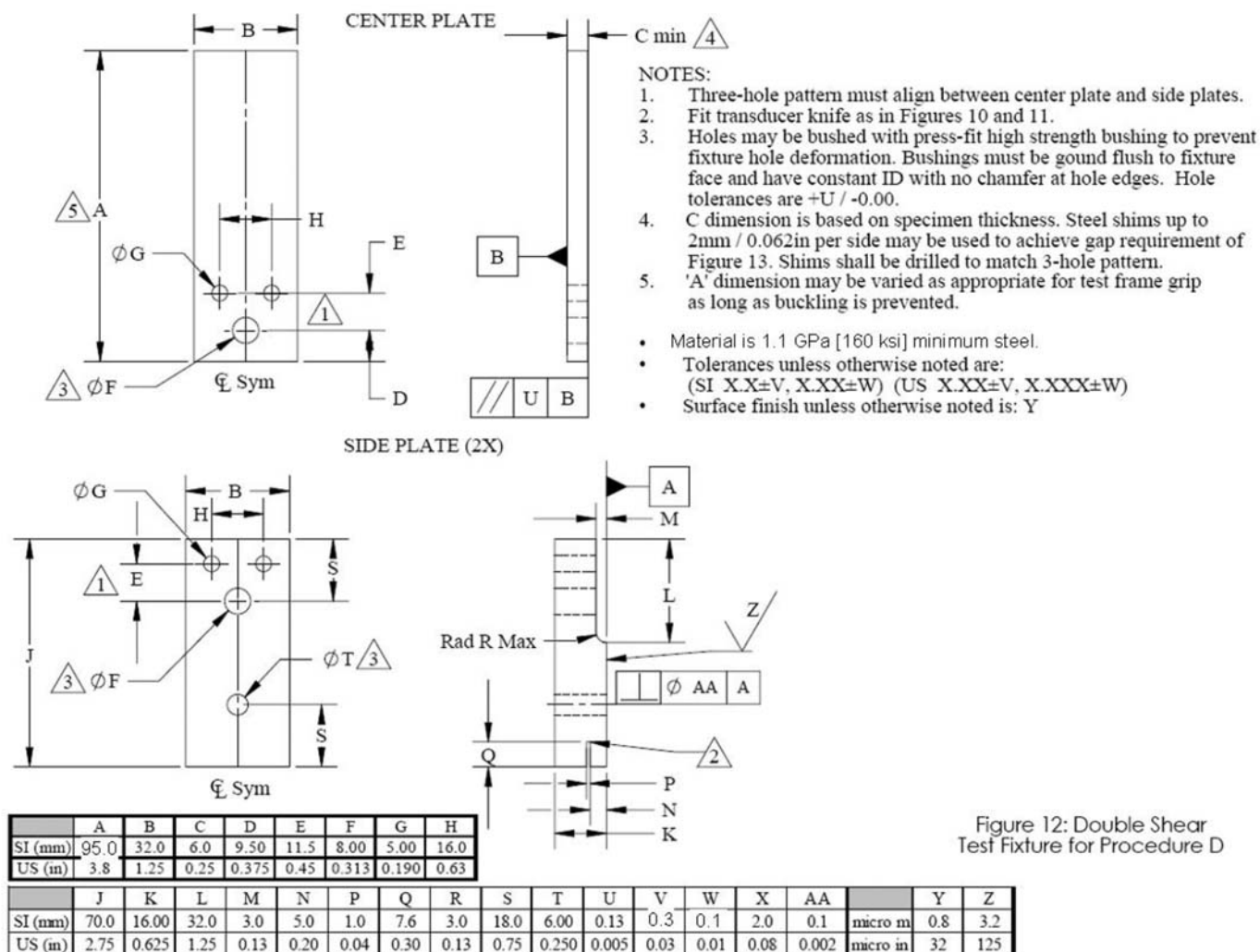
FIG. 12 Double-Shear Compression Test Fixture for Procedure D
