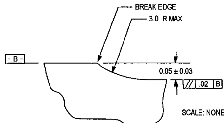
DETAIL B: RADIUS DETAIL
