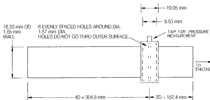
FIG. A3.1 Air Intake Piezometer Ring
