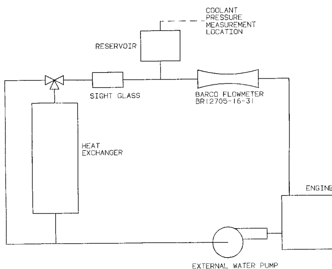
FIG. A3.4 Engine Coolant System
