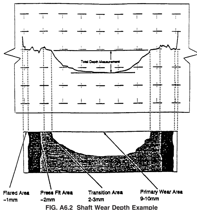
FIG. A6.2 Shaft Wear Depth Example
