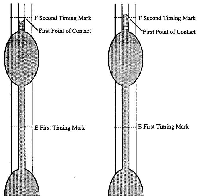
FIG. A3.4 Second Timing Mark
