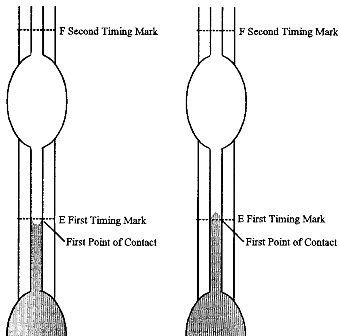
FIG. A3.3 First Timing Mark
