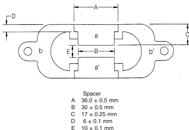
FIG. 1 Mold for Elastic Recovery Test Specimen
