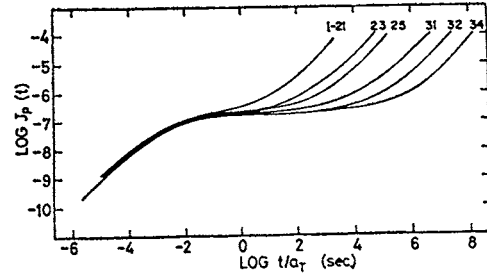
Master curves for creep compliance of polyisoprene of different molecular weights at a reference temperature of -30^{\circ}\text{C} :
