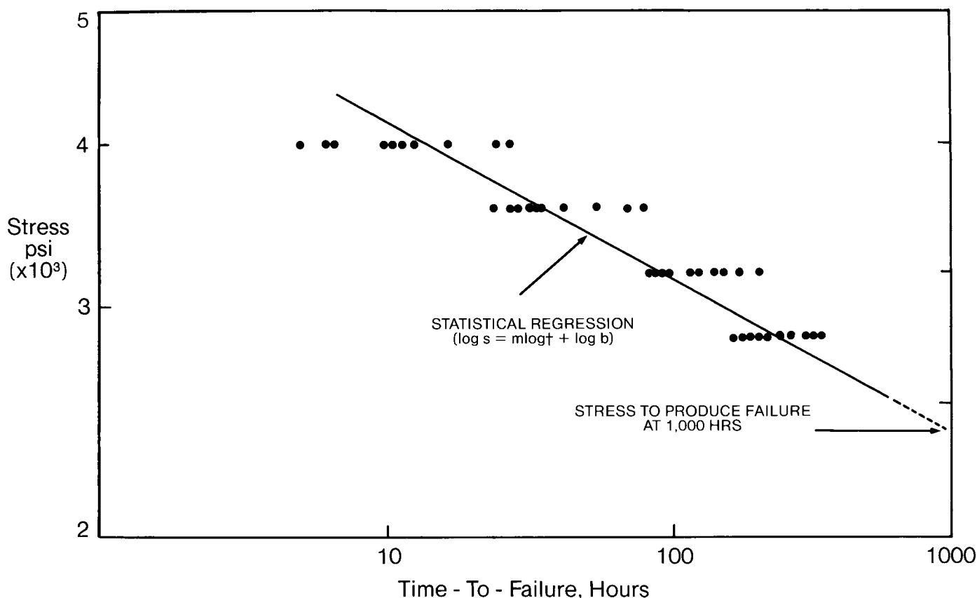
FIG. 4 Logarithmic Time-to-Failure (Stress Rupture) Curve
