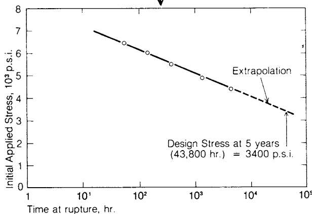
Fig. 1. Creep rupture of SAN at 73° F., extrapolated to obtain design stress at 5 years.
