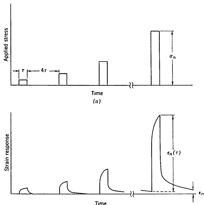
FIG. X4.2 Isochronous Data
