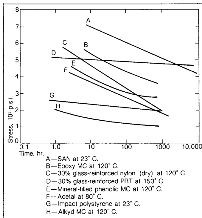
FIG. X3.4 Creep Rupture Envelope
