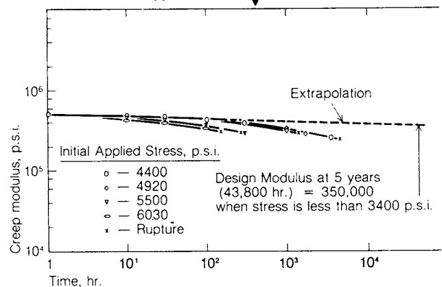
Fig. 2. Creep modulus of SAN at 73° F., extrapolated to obtain design modulus at 5 years.
