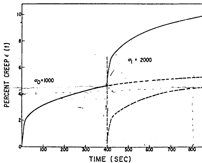
FIG. X5.1 Boltzmann Principle
