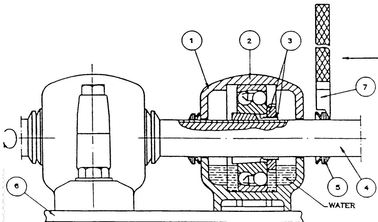
FIG. A1.1 Suitable Test Rig
