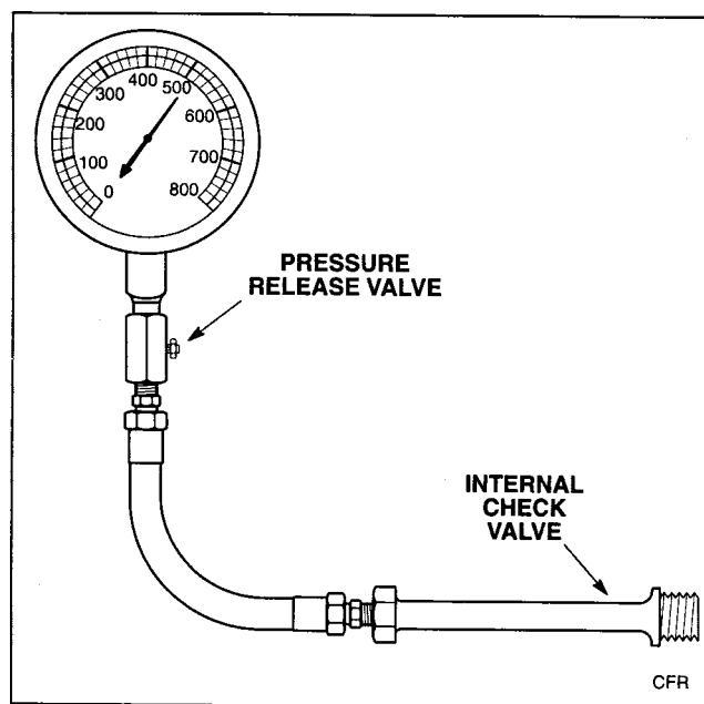
FIG. A2.2 Compression Pressure Gauge Assembly
