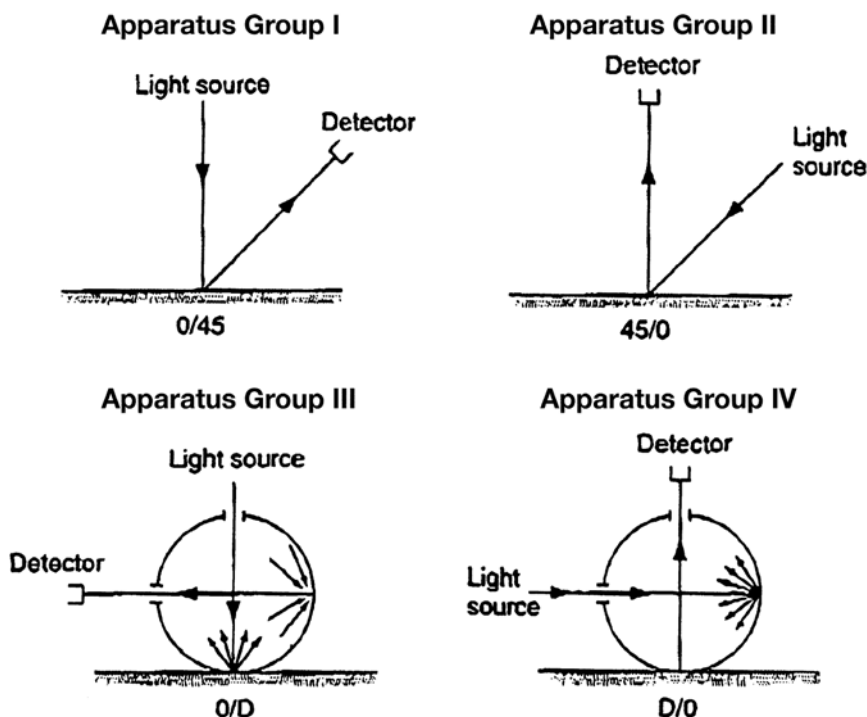
FIG. X1.1 CIE Recommended Illuminating and Viewing Geometries
