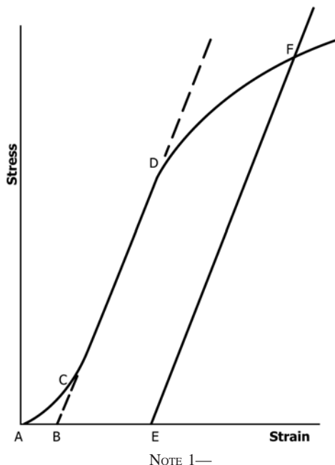
FIG. A1.1 Material with Hookean Region
