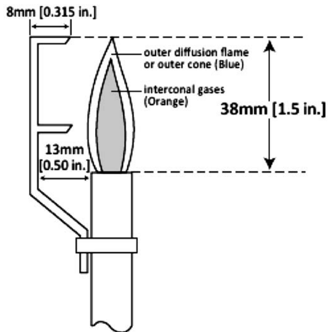
FIG. 6 Flame Height Adjustment
