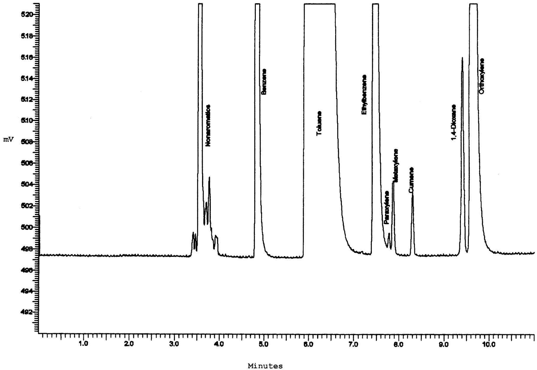
FIG. 1 Low Purity Toluene Sample Chromatogram
