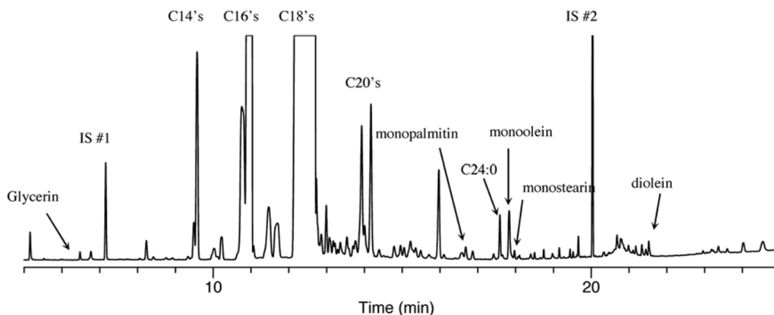
FIG. X1.6 Mixed feedstock based B100 example chromatogram
