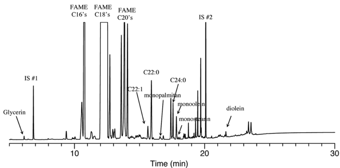
FIG. X1.4 Canola based B100 example chromatogram
