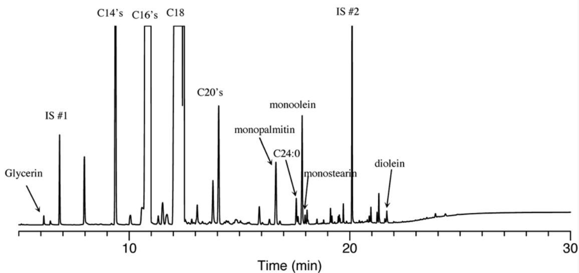
FIG. X1.5 Palm based B100 example chromatogram
