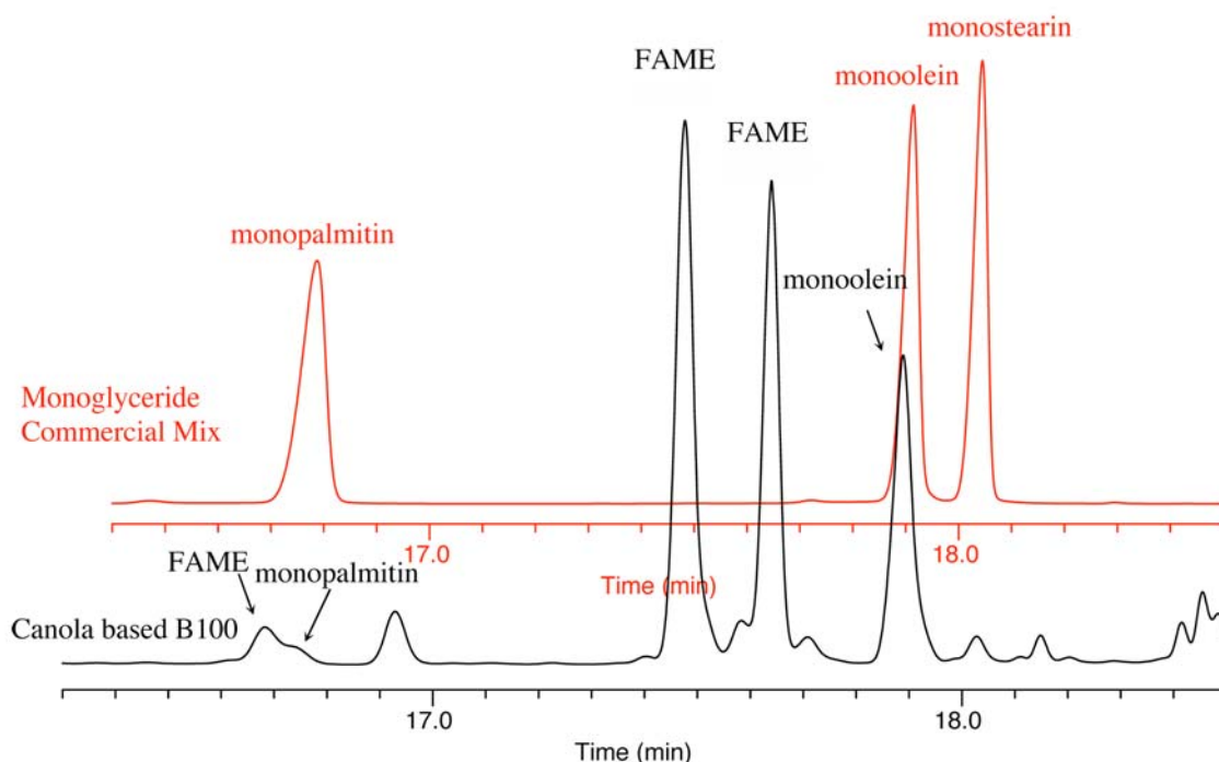
FIG. X1.1 Overlay of Canola based B100 and Monoglyceride Standard Solution
