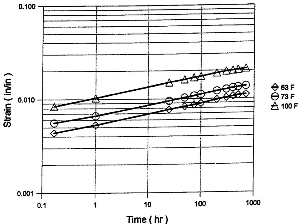
FIG. X1.4 Effect of Temperature on Flexural Creep of Plastic Lumber on a Log-Log Plot
