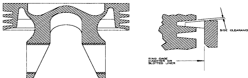
FIG. A10.2 Piston and Ring Specifications
