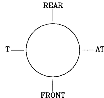
FIG. A13.2 Liner Thrust and Anti-Thrust Locations
