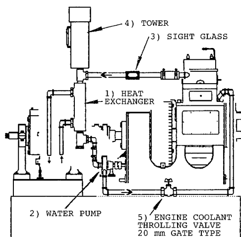
FIG. 8 Cooling System
