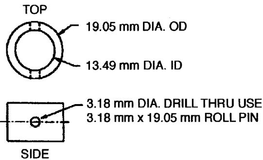
FIG. A10.6 Modified Ford Distributor-Upper Collar
