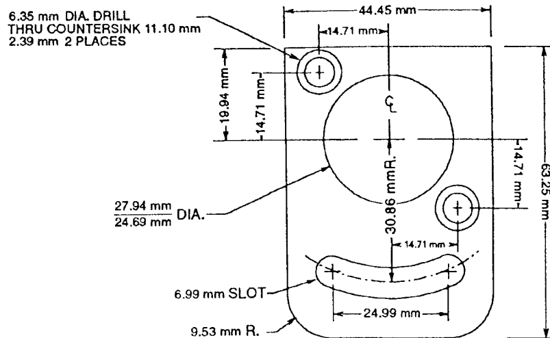
FIG. A10.8 Fabricated Hold Down Clamp
