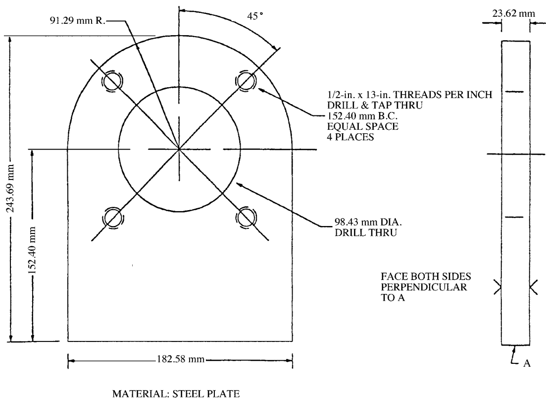
FIG. A6.1 Stress Plate
