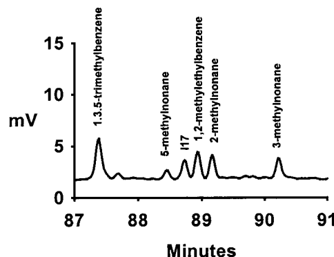
FIG. 8 I17 (unknown)/1,2-methylethylbenzene
