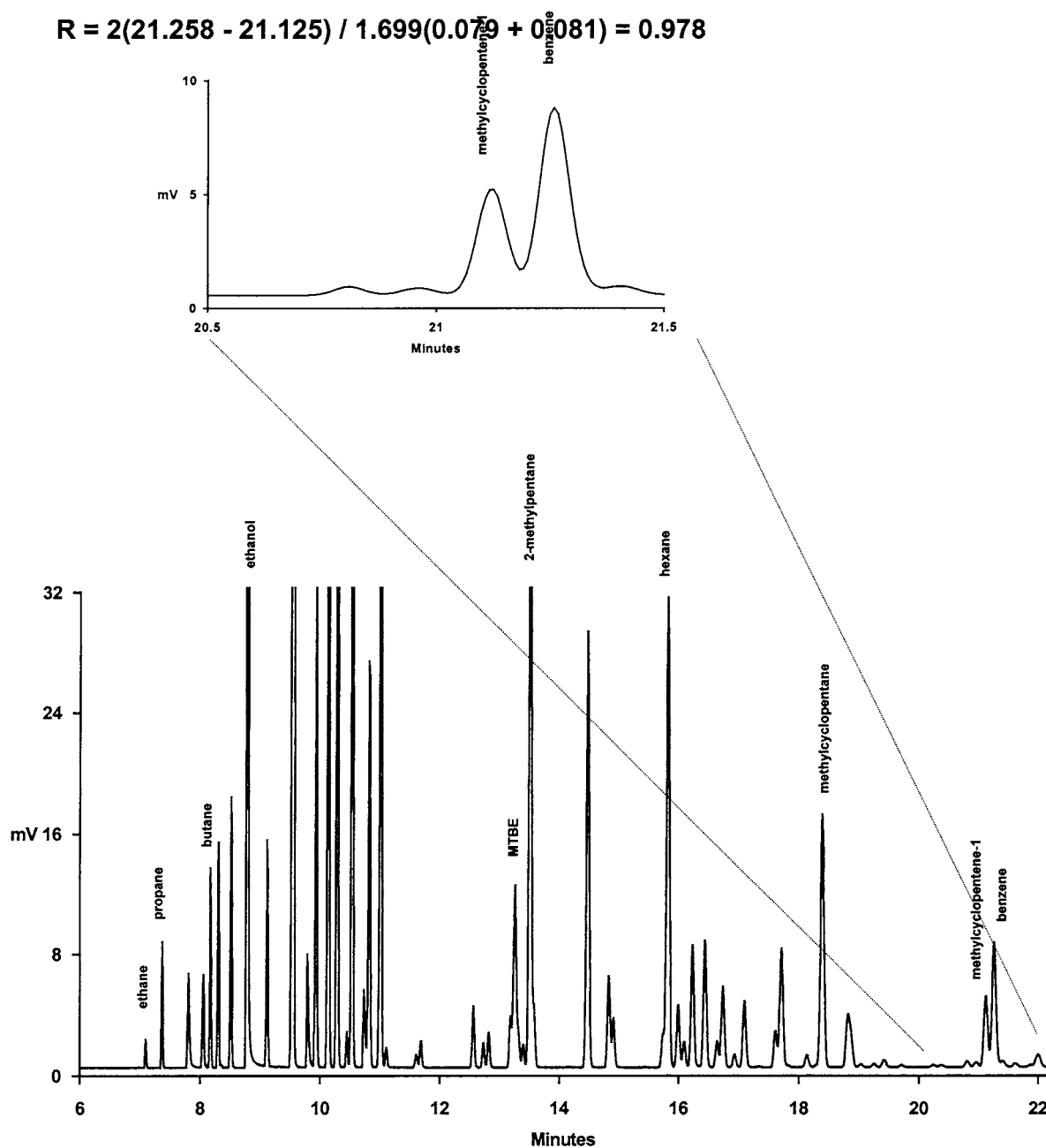
FIG. A1.7 PONA-V Standard - Analysis through Benzene New DHA Column plus 2 m x 0.25 mm 1 µm Precolumn Analyzed at 35 °C Isothermal
