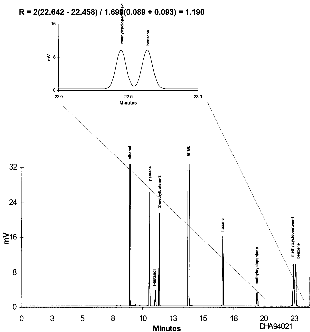
FIG. A1.8 DHA Calibration Standard - Analysis through Benzene New DHA Column plus 3 m x 0.25 mm 1 \mu m Precolumn Analyzed at 35 ^{\circ} C Isothermal
