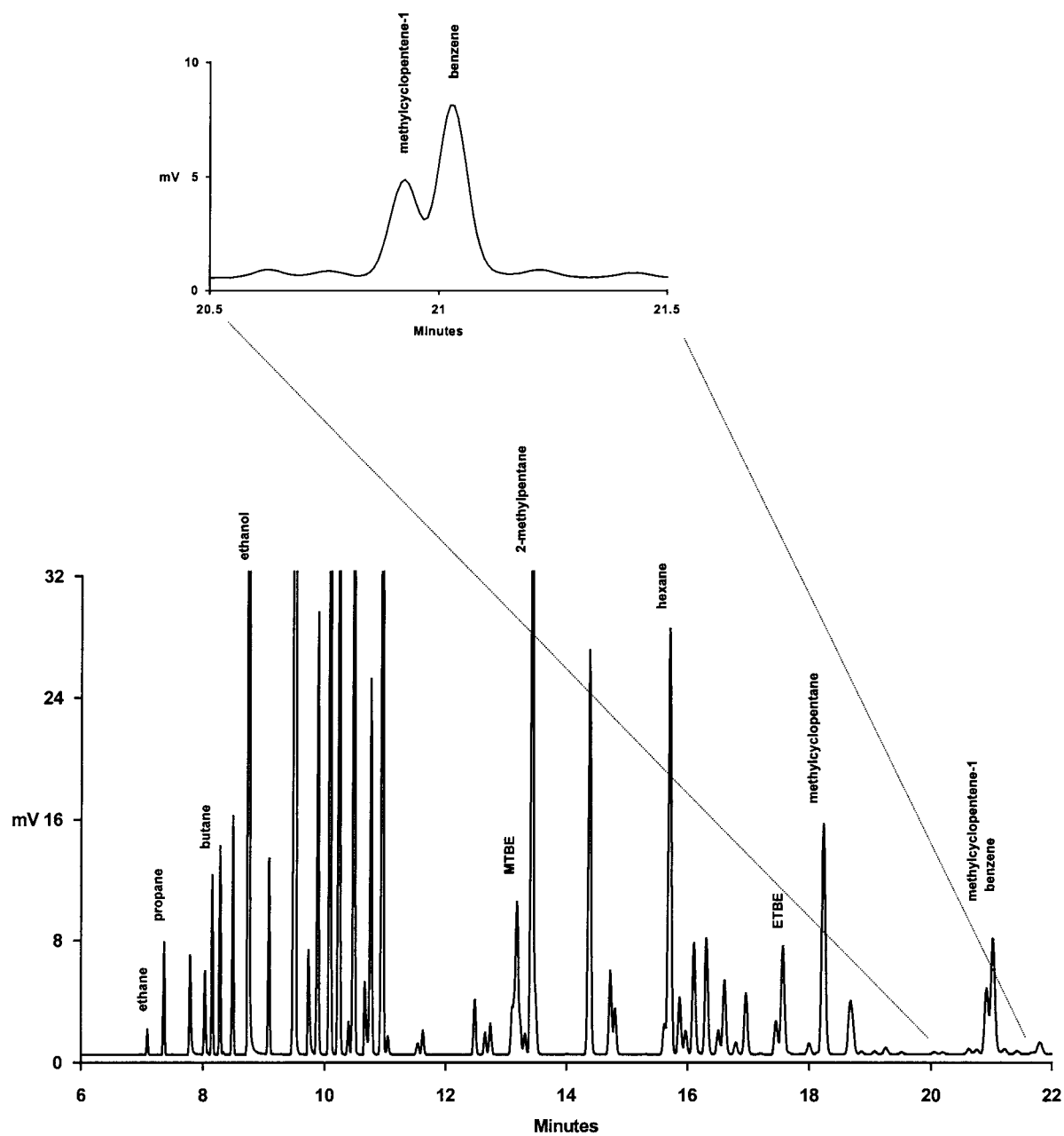
FIG. A1.6 PONA-V Standard - Analysis through Benzene New DHA Column plus 1 m x 0.25 mm 1 µm Precolumn Analyzed at 35 °C Iso-thermal
