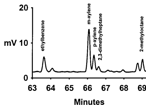
FIG. 7 p -xylene/2,3-dimethylheptane
